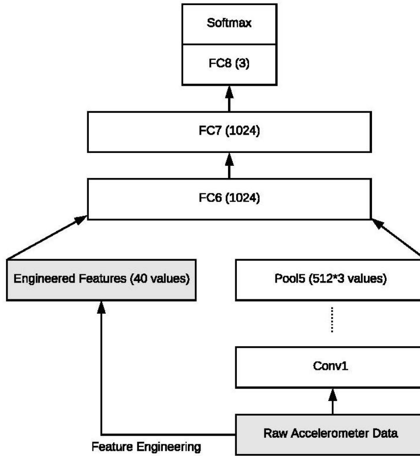
Supplementary Figure 1. Architecture of the Wide Convolutional Neural Network model.
